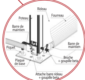
Tension rideaux
