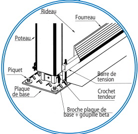
Tension rideaux
