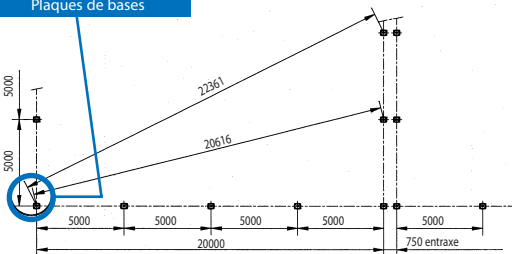
Implantation
